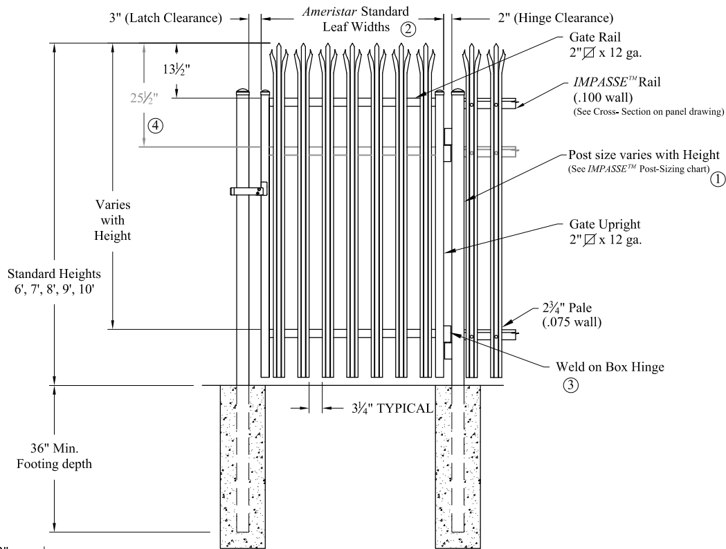
Single gate Arrangement
