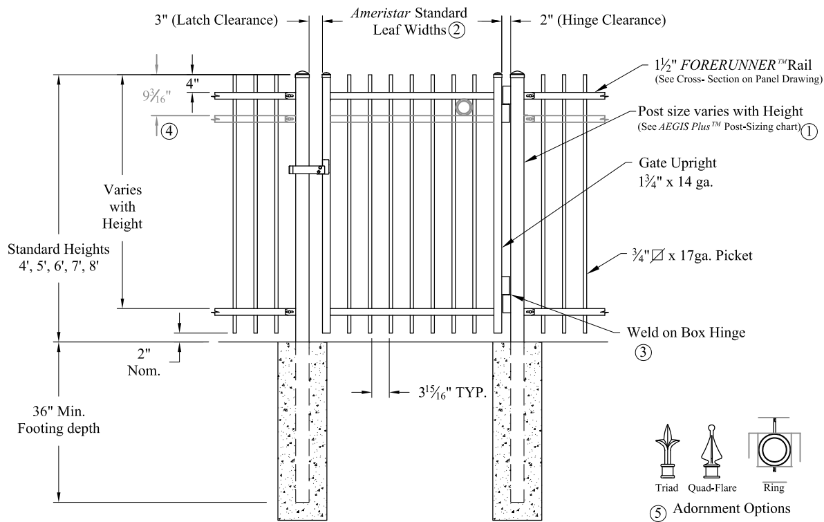
Single gate Arrangement
